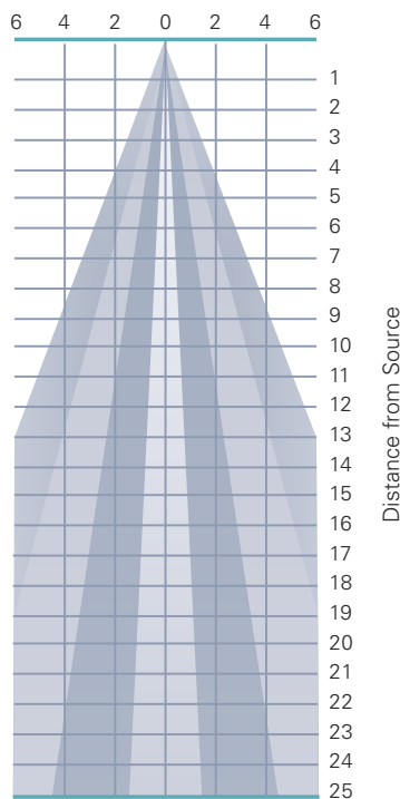
Photometric Data based on LED Rating: 19-80 (1856 Lumens/80CRI/19Watts)
