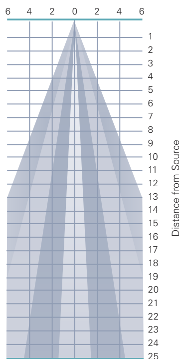
Photometric Data based on LED Rating: 15-90 (1500 Lumens/90CRI/18Watts)
