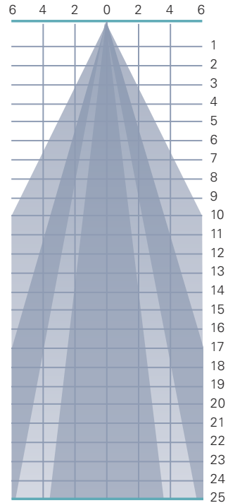
Photometric Data based on LED Rating: 13-98 (1300 Lumens/98CRI/29watts)
