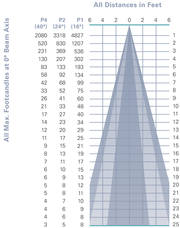
Photometric Data based on LED Rating: 10-92 (1000 Lumens/92CRI/15watts)
