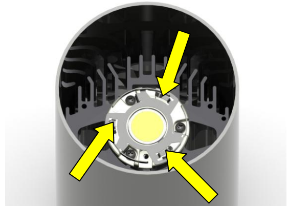
Figure 14. The three clips in the LED Adapter Ring. Align the reflector tabs with these clips and rotate clockwise to secure it in place.
