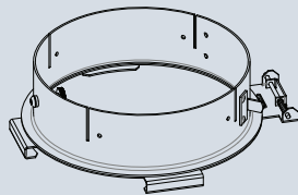
EXTERNAL ACCESSORIES CARTRIDGE LP1 External Accessory cartridge to hold LP1 hood and LP1 barndoor. Black finish.
