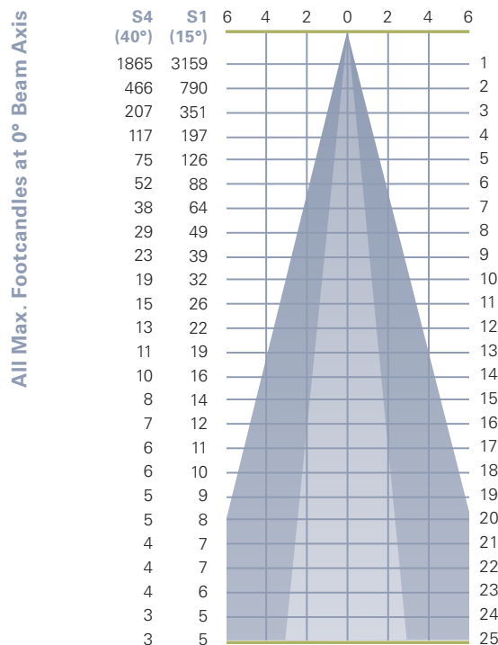
Photometric Data based on LED Rating: 11-83 (1100 Lumens/83CRI/11watts)
