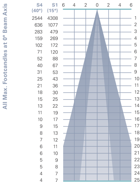
Photometric Data based on LED Rating: 15-83 (1500 Lumens/83CRI/14watts)
