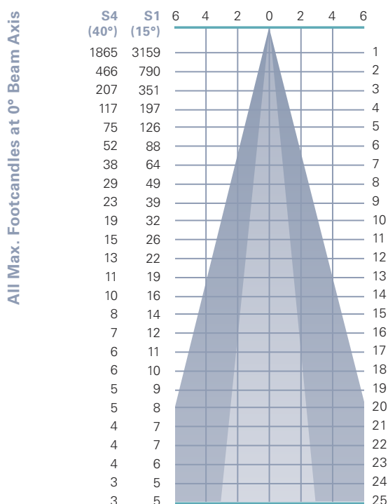
Photometric Data based on LED Rating: 11-83 (1100 Lumens/83CRI/11watts)
