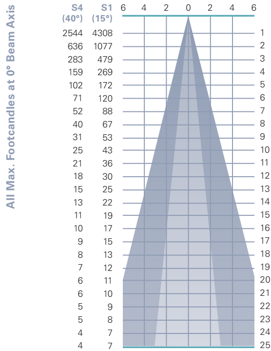
Photometric Data based on LED Rating: 15-83 (1500 Lumens/83CRI/14watts)
