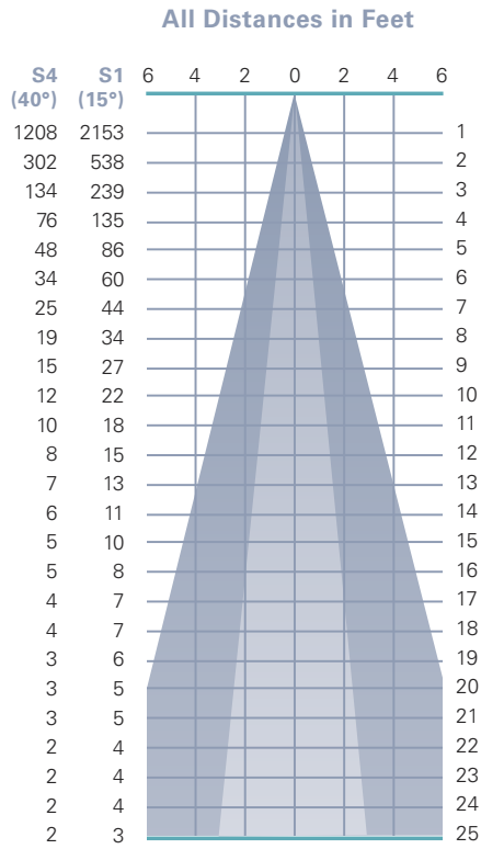
Photometric Data based on LED Rating: 08-90 (750 Lumens/90CRI/13watts)
