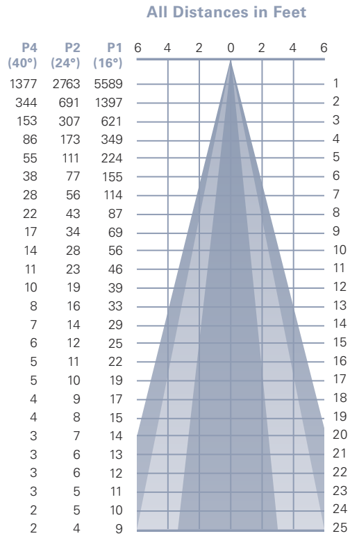
Photometric Data based on LED Rating: 09-83 (900 Lumens/83CRI/14watts)
